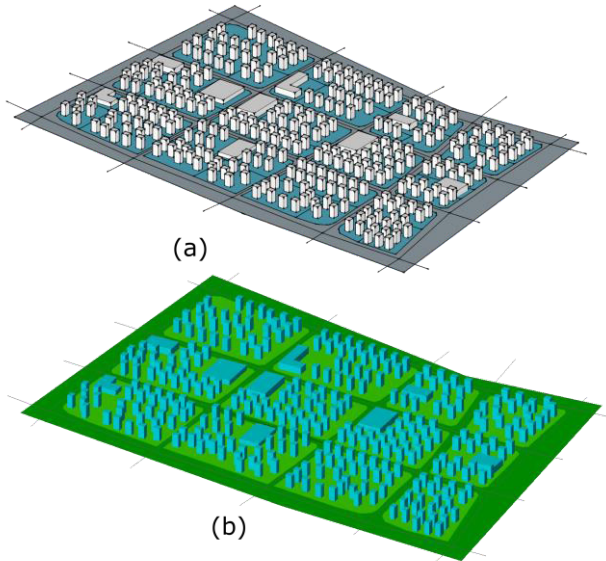
Fig. 4. Example 1 (a) SketchUp massing model (b) Converted CityGML model from the massing model
