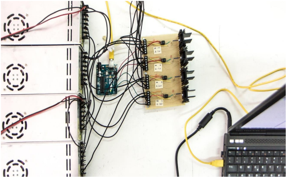
Fig. 4. Electronic circuit
